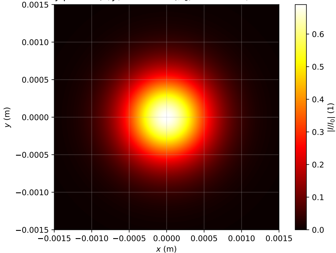
Intensity profile I(x, y, z = 2.946m)/I_0 , P_{in}=0.6P_{cr} , artificial time
